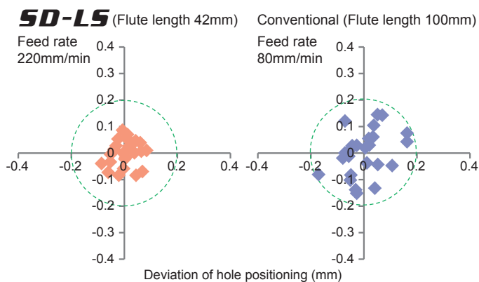
Deviation of hole positioning in surface machining
