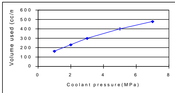
Dia.6: Relationship between coolant pressure and the volume used.
